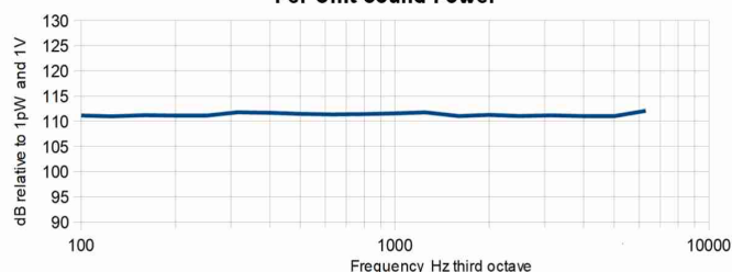
Output reference Voltage Per Unit Sound Power
