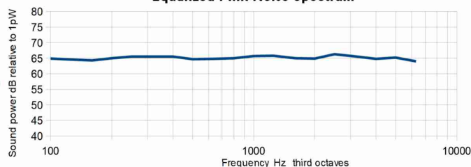
Equalized Pink Noise Spectrum
