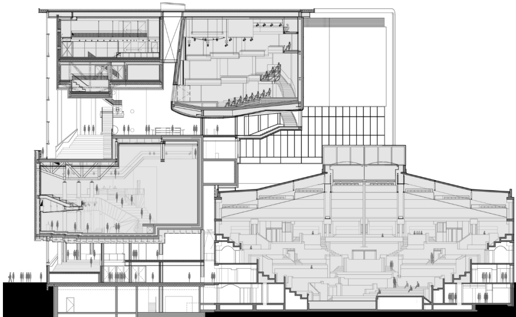
Figure 4. Cross-section of the concert hall
